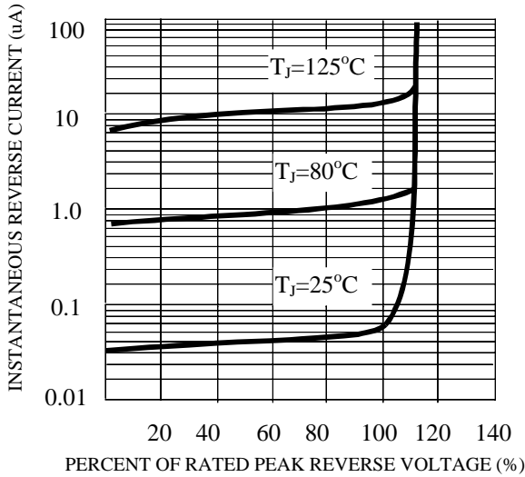
FIG. 3-TYPICAL REVERSE CHARACTERISTICS
